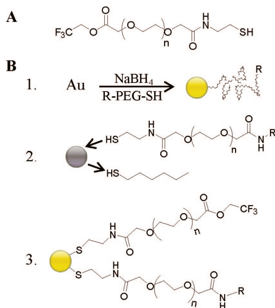
SCHEME 3. General Routes for Use of TFEF–PEG–SH for the Functionalization of Nanoparticles a
