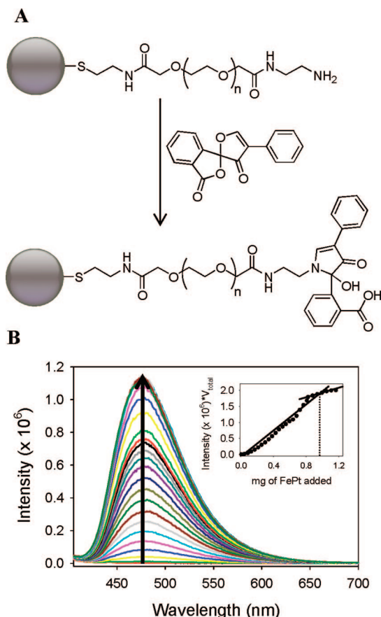
FIGURE 4. (A) Reaction of \text{H}_2\text{NC}_2\text{H}_4\text{NH}-\text{PEG}-\text{SH} -substituted FePt nanoparticles with fluorescamine and (B) fluorescence emission spectra of a dichloromethane solution containing 0.02 \mu\text{mol} of fluorescamine during the sequential addition of 20 \mu\text{L} aliquots of \text{H}_2\text{NC}_2\text{H}_4\text{NH}-\text{PEG}-\text{SH} -modified FePt particles ( 1.42 \text{ mg/mL} ). Excitation wavelength is 390 \text{ nm} . The inset shows emission intensity at 475 \text{ nm} vs quantity of added FePt particles.
