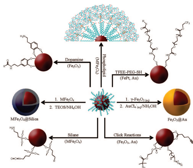
SCHEME 2. Selected Functionalization Routes for Magnetic Nanoparticles
